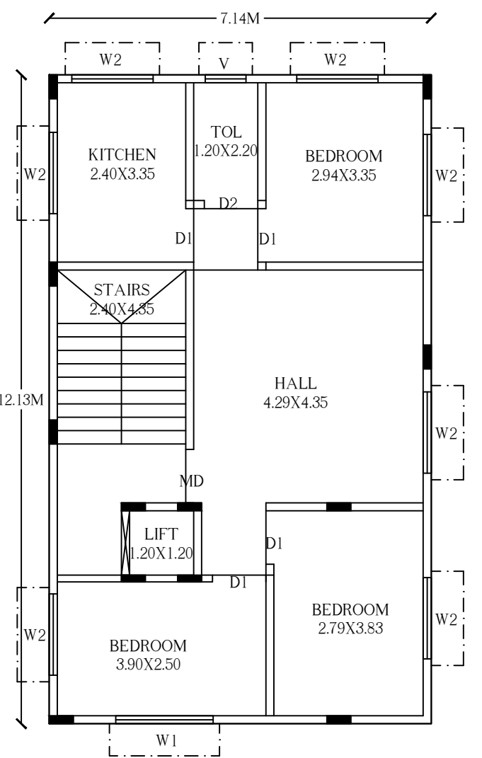
TYPICAL GROUND, FIRST & SECOND FLOOR PLAN
